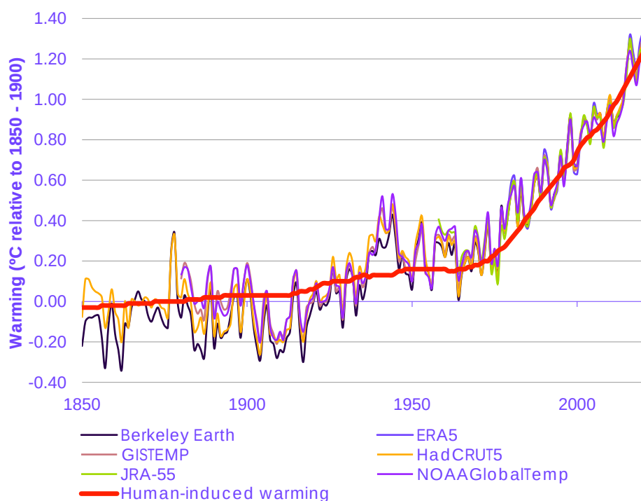
Figure 1.1 Global average surface air temperature change
