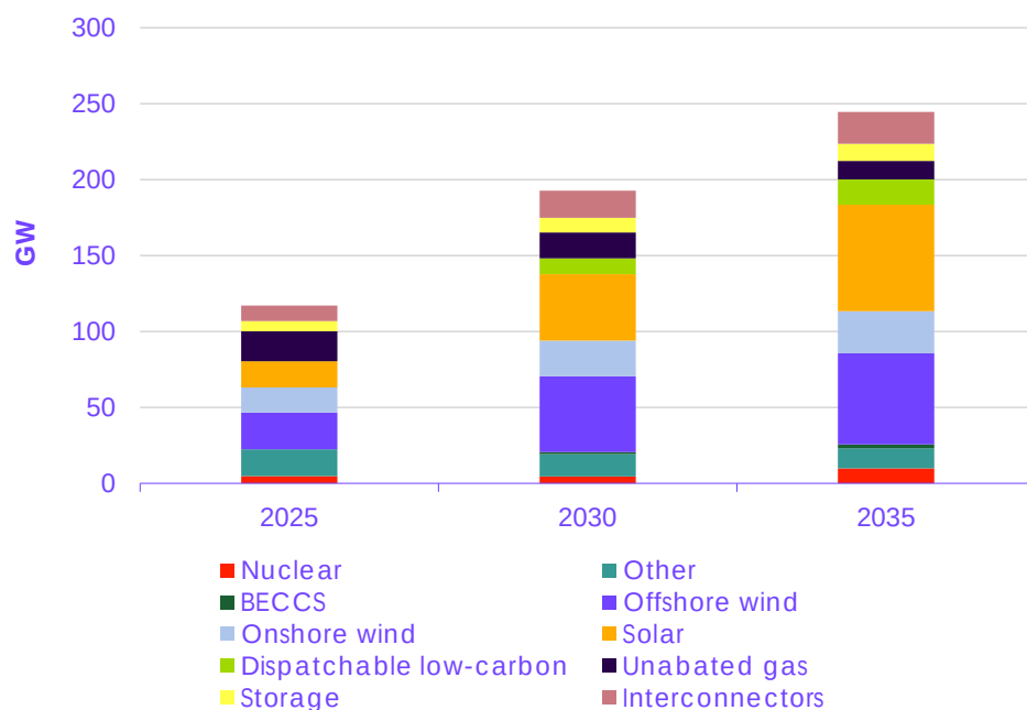
Figure 6.3 Electricity capacity mix to 2035 in the Central scenario
