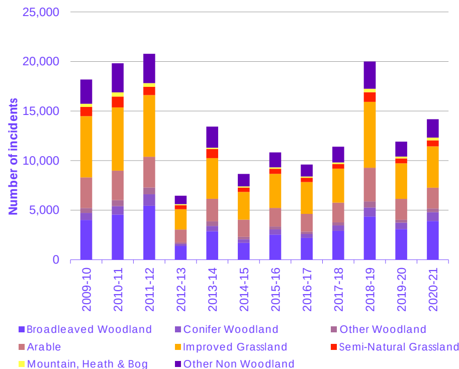
Figure 2.4 Total number of wildfire incidents in England per annum, split by land cover class.
