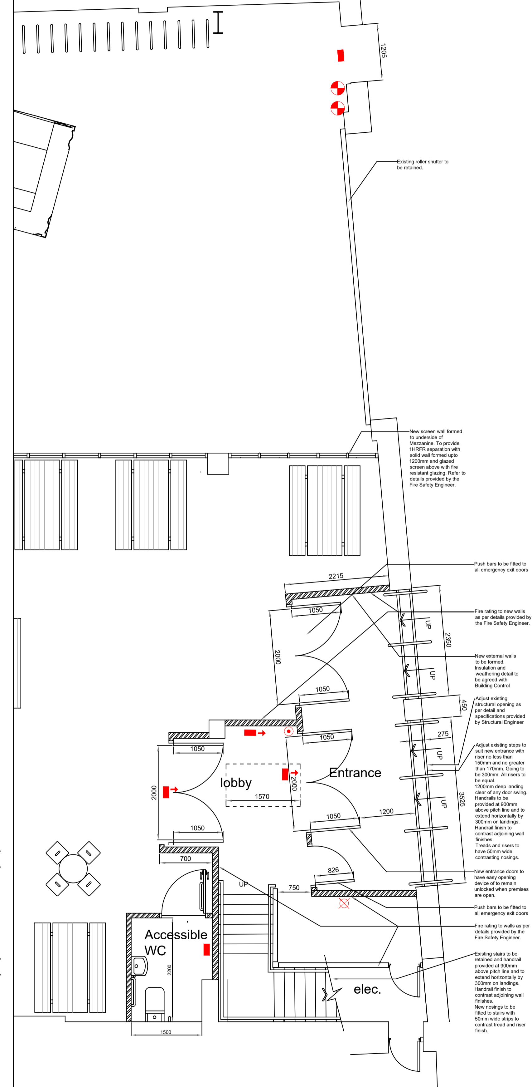
Proposed Ground Floor Entrance Detail Plan
